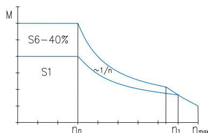
TORQUE DIAGRAM
